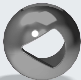
V-NOTCH ANGLE 60°
